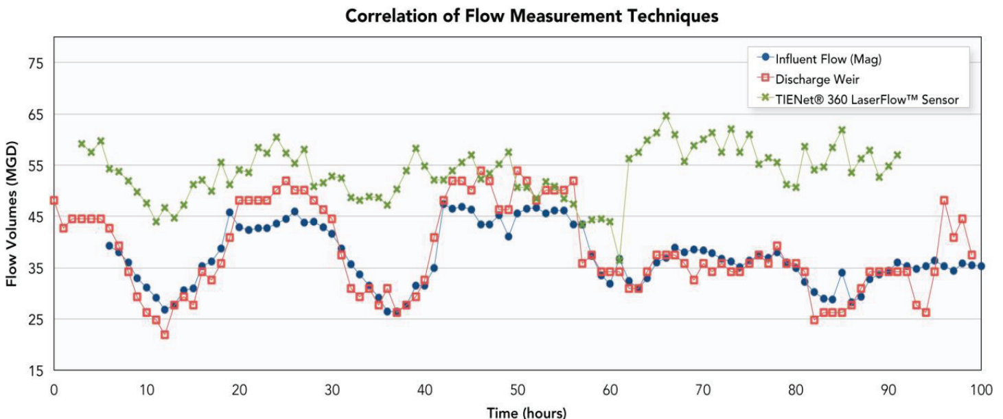
FIGURE 1. Correlation of the three effluent volume measurements
