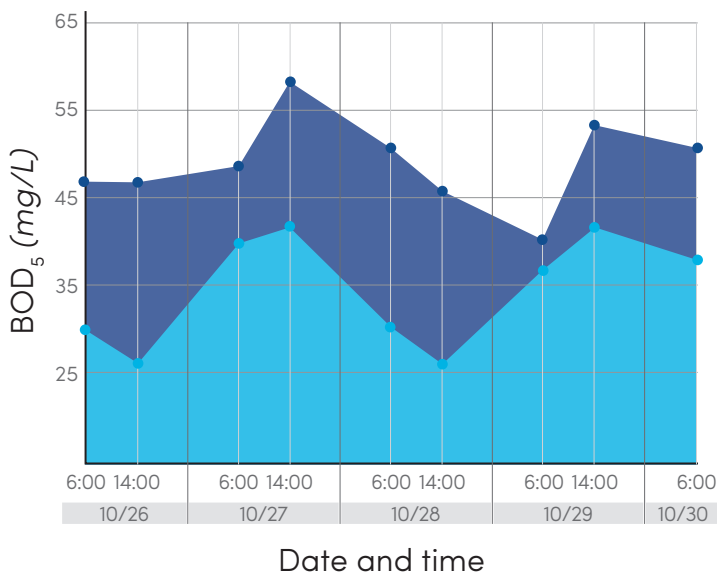
FIGURE 3. BOD 5 comparison in the treated and untreated effluent wastewater
