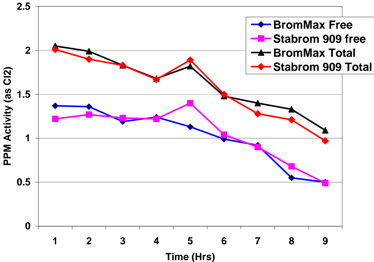
Relative Stability of BromMax™ and Stabrom™ In Synthetic Cooling Water @ pH 8.8
